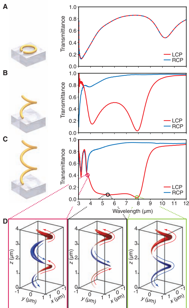
Fig. 1. Connection between split-ring resonators (SRRs) and metal helices. The 2 \times 2 \mu\text{m} unit cells with 2 \mu\text{m} helix pitch used in the calculations in (A) to (C) are shown in the left column, normal incidence transmittance spectra for light impinging from the air side (no analyzer behind sample) in the right column. RCP and LCP refer to right and left-handed circular polarization of the incident light, respectively. (A) Planar SRR. Here, the RCP and LCP spectra are indistinguishable. (B) Adiabatically pulling the metal wire of an SRR out of the substrate plane leads to one pitch of a (left-handed) metal helix. (C) Two helix pitches (left-handed). (D) Snapshots of the electric current distribution along the metal wire for the three wavelengths [open dots in (C)]. The absolute value of the current is encoded by the curve thickness, the sign by red and blue (see arrows).
