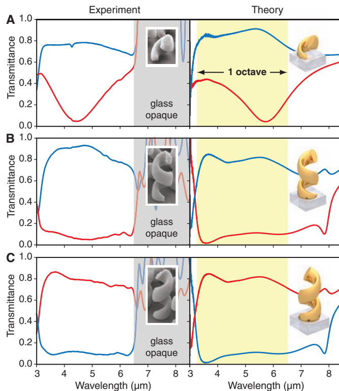
Fig. 4. Normal-incidence measured and calculated transmittance spectra (no analyzer behind sample) are shown in the left and right columns. LCP and RCP are depicted in red and blue, respectively. (A) Slightly less than one pitch of left-handed helices, and (B) two pitches of right-handed helices (see insets). For wavelengths longer than 6.5 \mu\text{m} , the glass substrate in the experiments becomes totally opaque. Hence, transmittance cannot be measured. For wavelengths below 3 \mu\text{m} , light can be diffracted into the glass substrate ( a = 2 \mu\text{m} and refractive index n = 1.5 ), giving rise to Wood anomalies.
