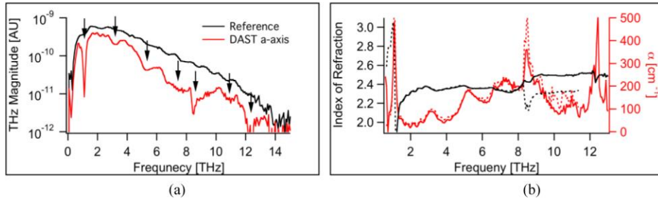
Fig. 3. (a) Broader bandwidth THz spectroscopy clearly identifying seven absorption bands. (b) The new data set (solid) overlaps previous data (dashed) but experiences an artificial kink in the index of refraction at the 8.4 THz absorption feature, due to the saturation of this absorption feature.
