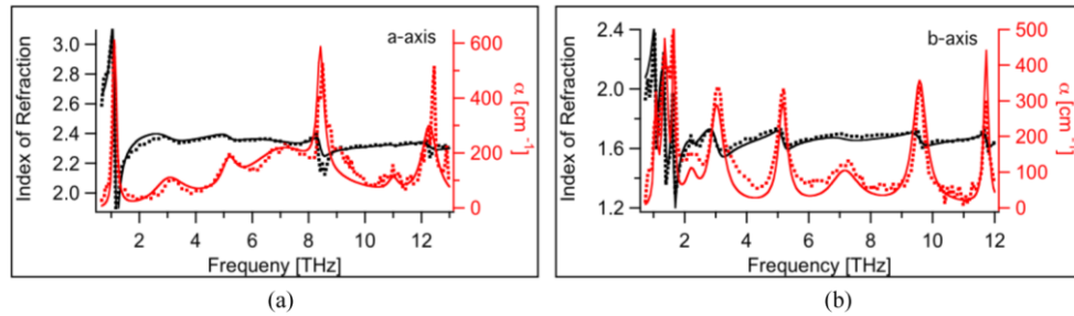
Fig. 4. Composite refractive index and absorption coefficient of the (a) a - and (b) b -axis of DAST from 0.6 – 12 THz. The solid lines are fits to the Lorentz oscillator model described in the text.
