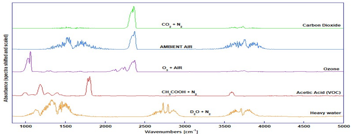
Gas spectra examples measured with Gasex system.
