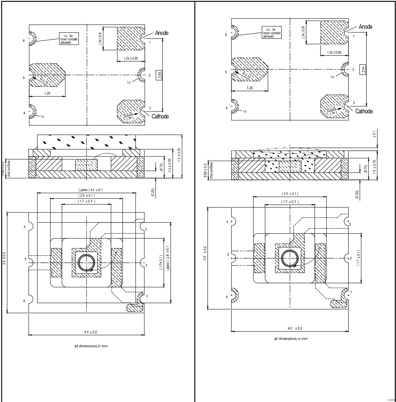
Technical Drawing, Package: LCC6.1 LCC6.1G with glass cover # 3001210
