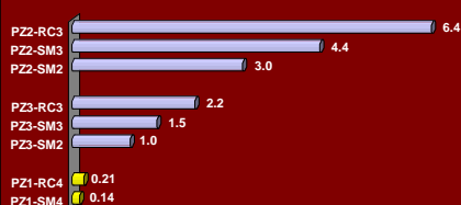
Relative SM Fiber Stretch at max. drive (P-P) in nm
