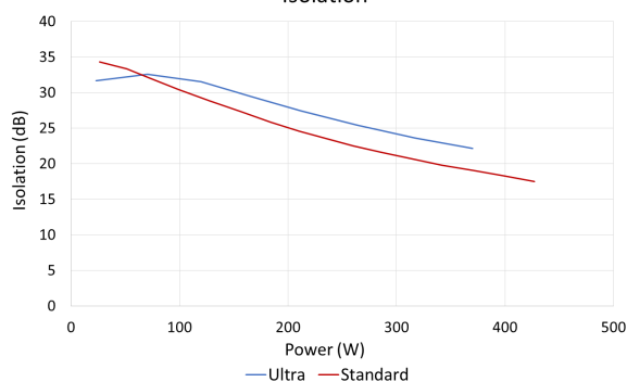
Isolation
