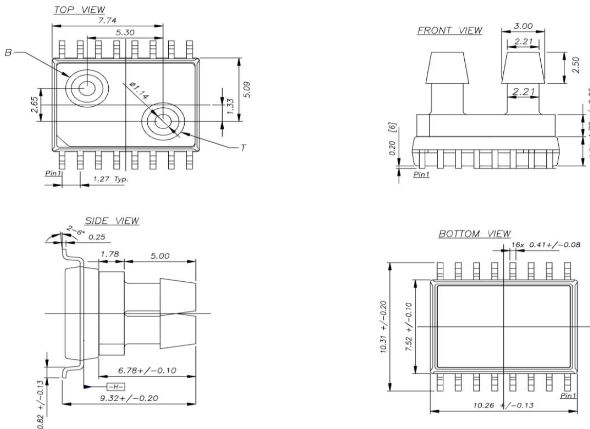
SOIC-16 (C) Vertical Package Dimensions
