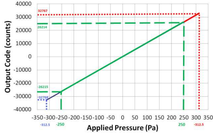
An example for a 250 differential SM9336-BCE-S-250-000 is given in the graph below SM933X-250 Pa: Count vs. Pressure
