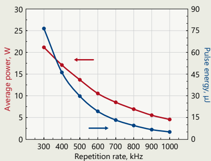
Fig 8. Typical output power and energy curves of Atlantic 50-UV18
